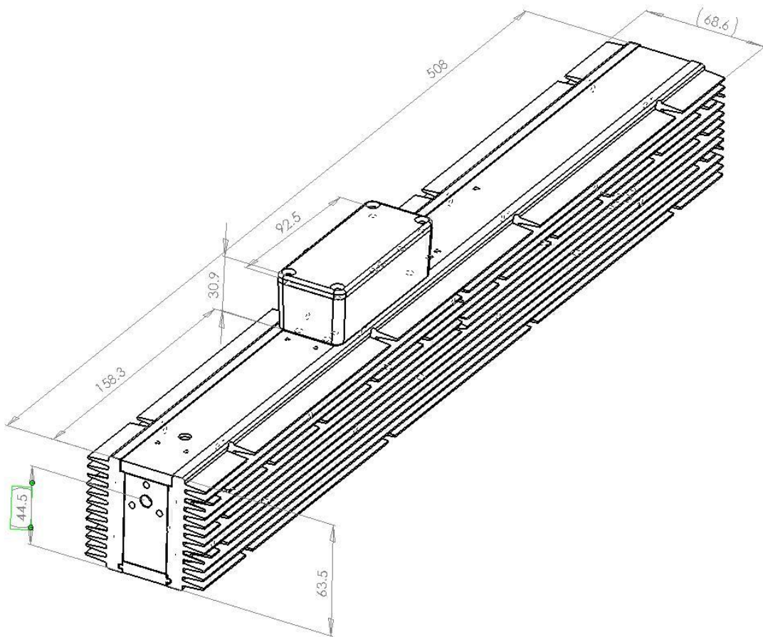
Mounting Illustration, Top View, Units in mm
